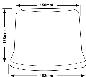
Outer housing dimensions
